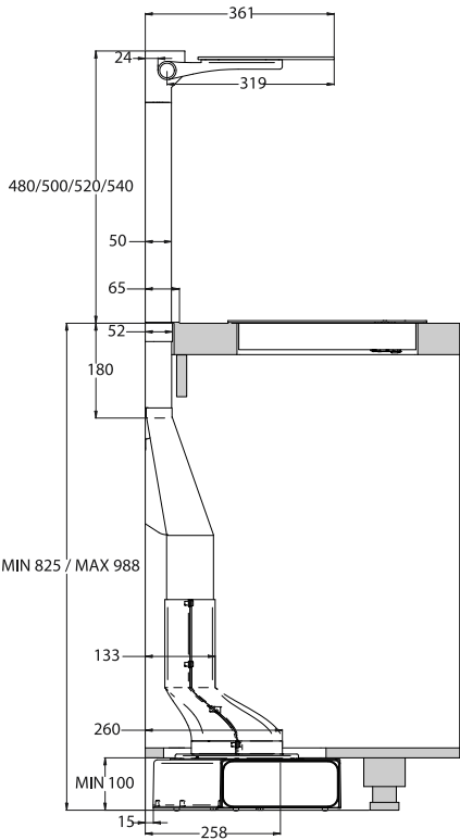
Vista laterale Side view
