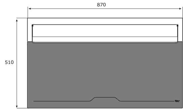
Foratura top Built-in cutout for top
