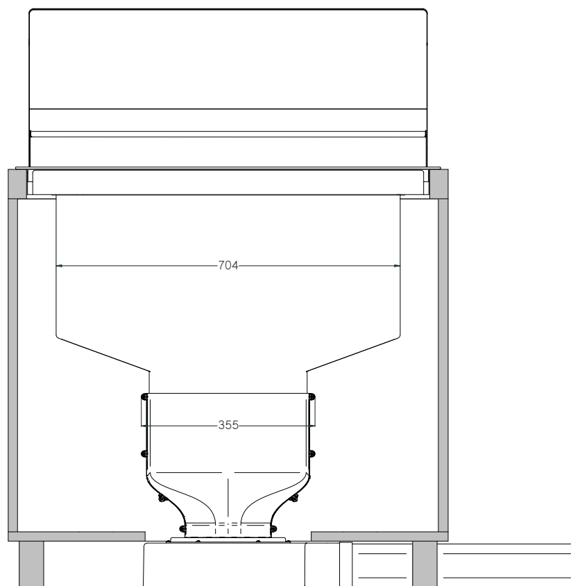
Vista frontale Front view
